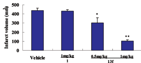
Figure 4. Effects of 1 (1 mg/kg, sc) and 13f (0.5 and 1 mg/kg, sc) on the infarct volume of ischemic damage in the transient MCA occlusion model. The bifurcation of the left common carotid artery was exposed, and the right MCA was occluded by insertion of a silicon-coated nylon suture (USS-DG, Dermalon) through the common carotid artery. After closure of the operative sites, the animals were temporarily transferred to a cage with a heating lamp and the suture was gently removed at 1.5 h after MCA occlusion. Drugs were dissolved in DMSO and subcutaneously injected 5 min after the start of MCA occlusion at a volume of 0.5 mL/kg. Transient occlusion of MCA for 1.5 h resulted in tissue damage 24 h after occlusion. Each column and vertical bar represents the mean \pm SE of results from eight rats. The operated animals showed statistical significance at P < 0.01 compared with saline-treated animals (one-way ANOVA followed by Dunnett's post hoc comparison).
