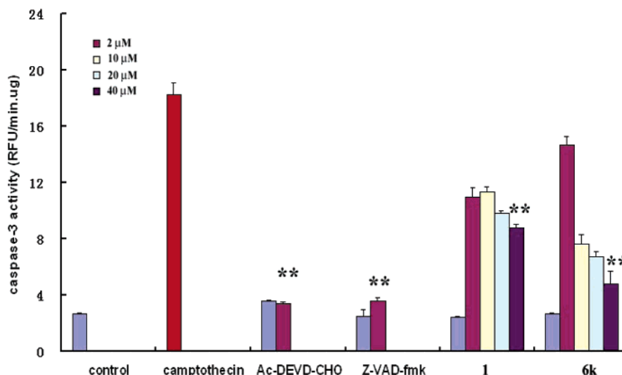
Figure 2. Concentration-dependent inhibition of caspase activity (Ac-DEVD-AMC) in camptothecin-induced apoptotic Jurkat T cells by caspase-3 inhibitors 1 and 6k . After treatment with 2 μM camptothecin only, caspase-3 activity increased from 2.7 ± 0.1 RFU (relative fluorescence unit) μg -1 min -1 (negative control) to 18.3 ± 0.7 RFU μg -1 min -1 in cell lysate. Treated with four caspase-3 inhibitors and camptothecin, caspase-3 presented a low activity compared with camptothecin only. The caspase-3 activities were 3.4 ± 0.1 and 3.6 ± 0.3 RFU μg -1 min -1 when treated with two positive inhibitors, Ac-DEVD-CHO (2 μM) and Z-VAD-fmk (2 μM), respectively. With 40 μM compounds 1 and 6k , the caspase-3 activities were 8.7 ± 0.3 and 4.8 ± 0.5 RFU μg -1 min -1 , respectively: (***) denotes P < 0.005 compared with camptothecin treatment alone.
