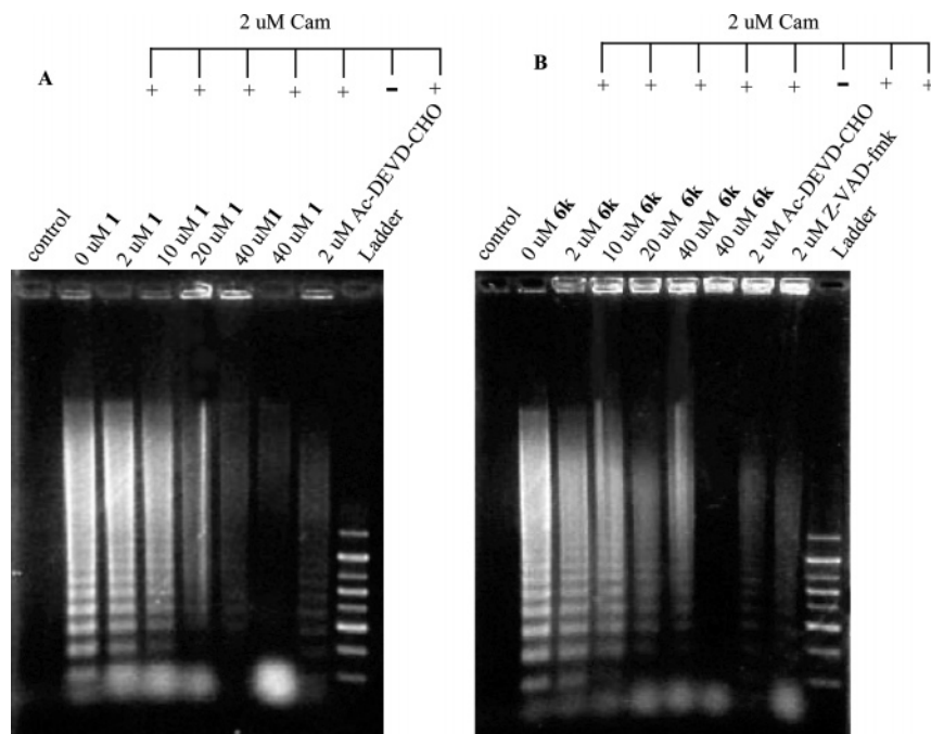
Figure 3. Detection of DNA fragments in Jurkat T cell apoptosis induced with camptothecin. (A) Compound 1 : lane 1, control cells without camptothecin; lanes 2–6, cells treated with 2 \mu M camptothecin and varying concentrations of inhibitors; lane 7, compound 1 only, without camptothecin; lane 8, positive control 2 \mu M Ac-DEVD-CHO with 2 \mu M camptothecin; lane 9, 100-bp DNA ladder used as standard. (B) Compound 6k : lane 1, control cells without camptothecin; lanes 2–6, cells treated with 2 \mu M camptothecin and varying concentrations of inhibitors; lane 7, compound 6k only, without camptothecin; lane 8, positive control 2 \mu M Ac-DEVD-CHO with 2 \mu M camptothecin; lane 9, positive control 2 \mu M Z-VAD-fmk with 2 \mu M camptothecin; lane 10, 100-bp DNA ladder used as standard.
